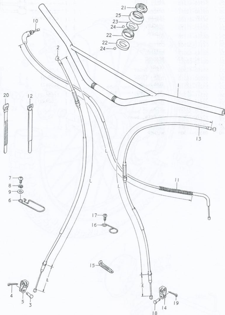
FIG. 36 HANDLEBAR (PE250B)
