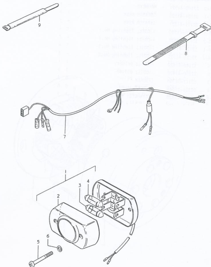
FIG. 54 FOR SPECIAL MARKET (E24)
