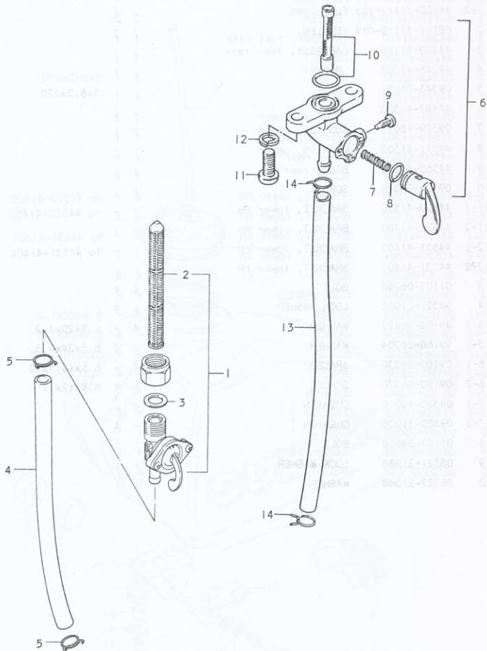
FIG.28 FUEL - COCK
