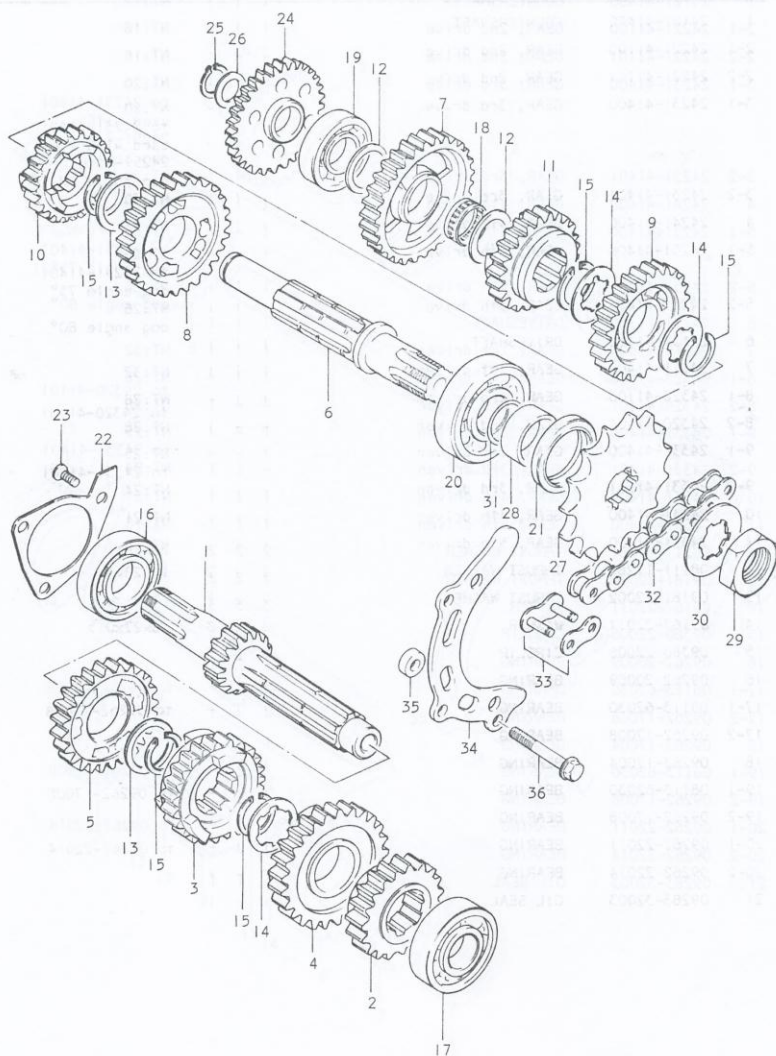
FIG.11 TRANSMISSION
