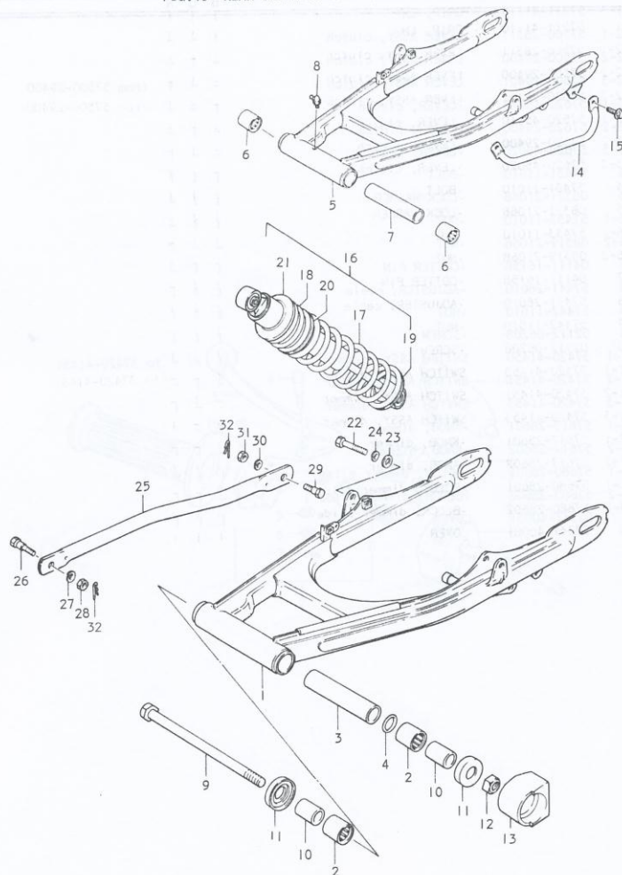
FIG.40 REAR SWINGING ARM (PE250B-PE250C)
