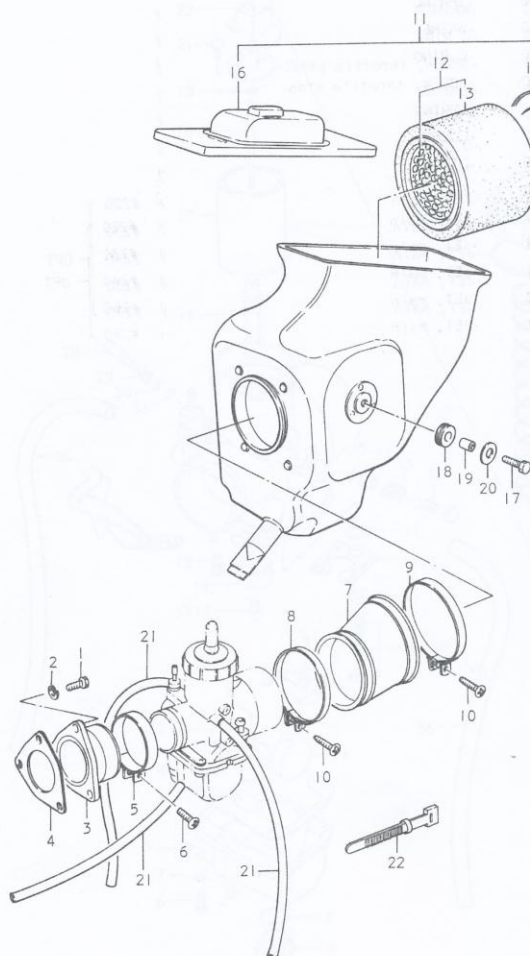
FIG.7 AIR CLEANER
