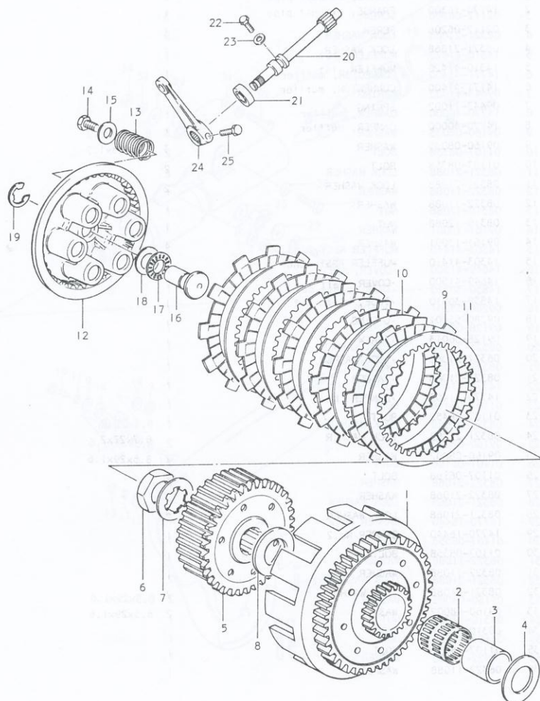
FIG.10 CLUTCH
