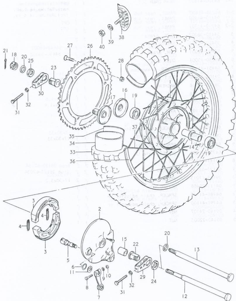
FIG.43 REAR WHEEL (PE250B·PE250C)
