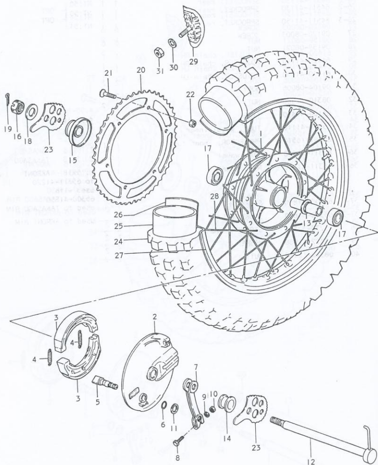
FIG.44 REAR WHEEL (PE250N)
