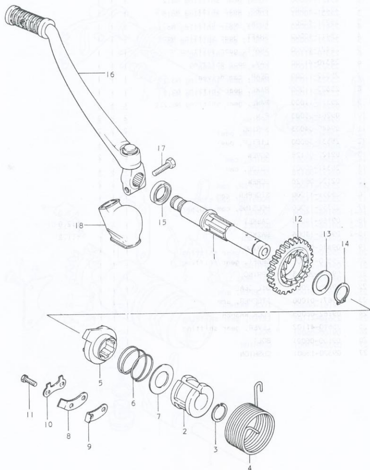
FIG.13 KICK STARTER
