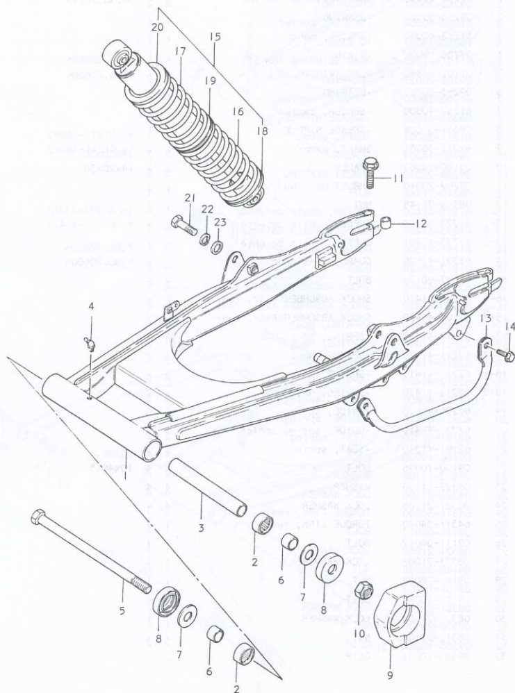
FIG.41 REAR SWINGING ARM (PE250N)
