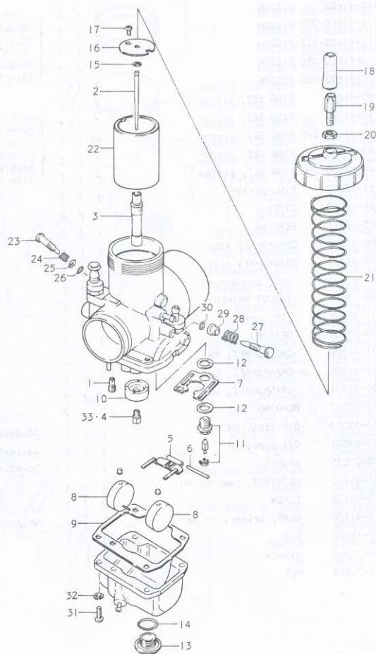
FIG.5 CARBURETOR (PE250B·PE250C)
