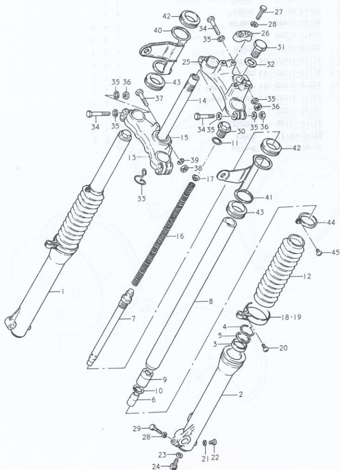
FIG. 30 FRONT FORK (PE250B)
