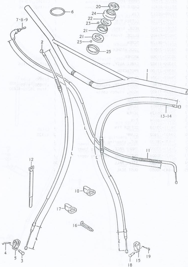
FIG.37 HANDLEBAR (PE250C·PE250N)
