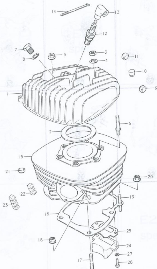
FIG.1 CYLINDER
