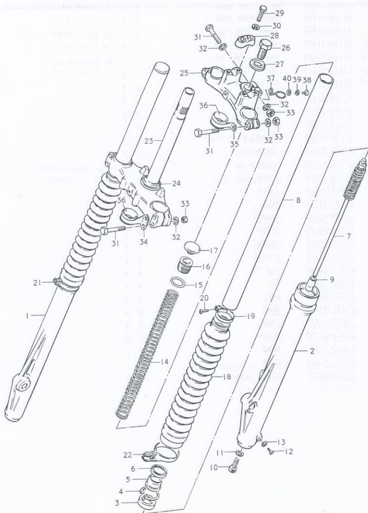
FIG.31 FRONT FORK (PE250C·PE250N)
