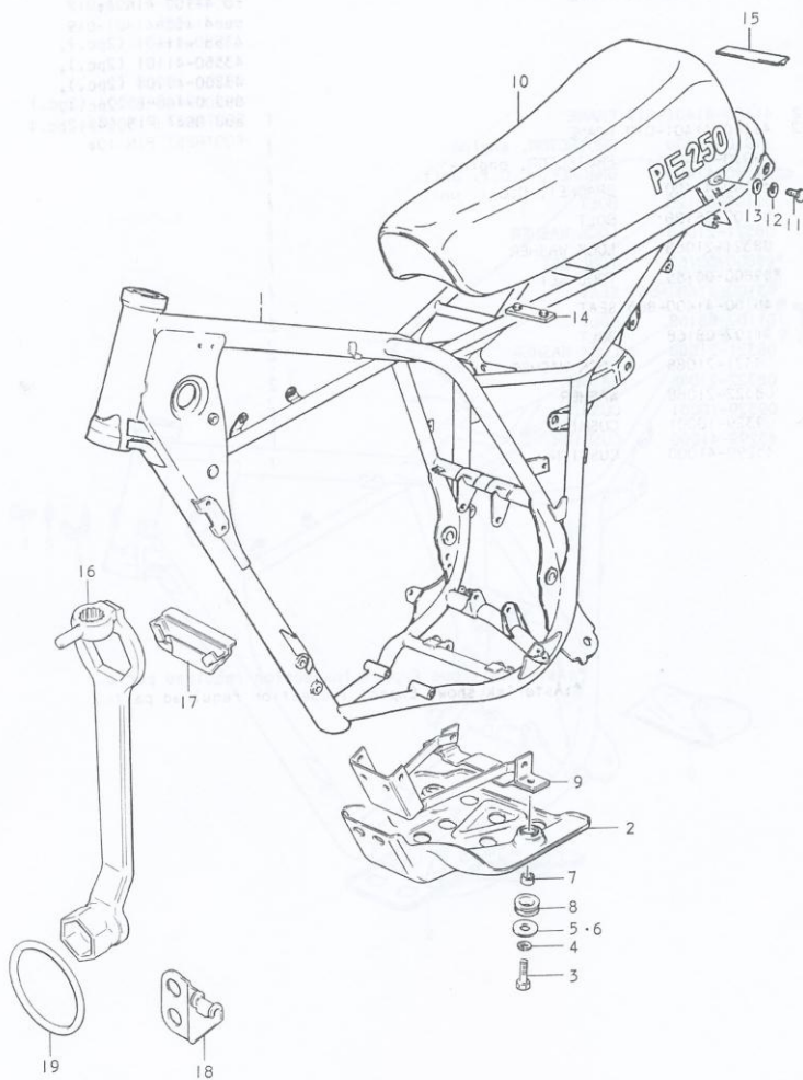
FIG.23 FRAME - SEAT (PE250C·PE250N)
