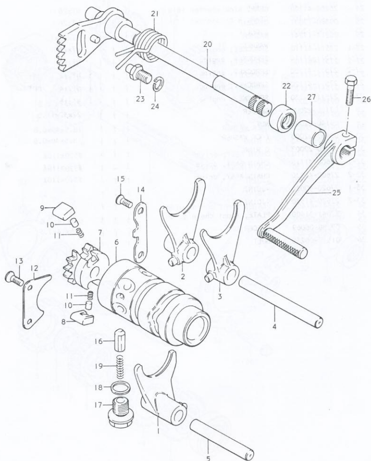
FIG.12 GEAR SHIFTING
