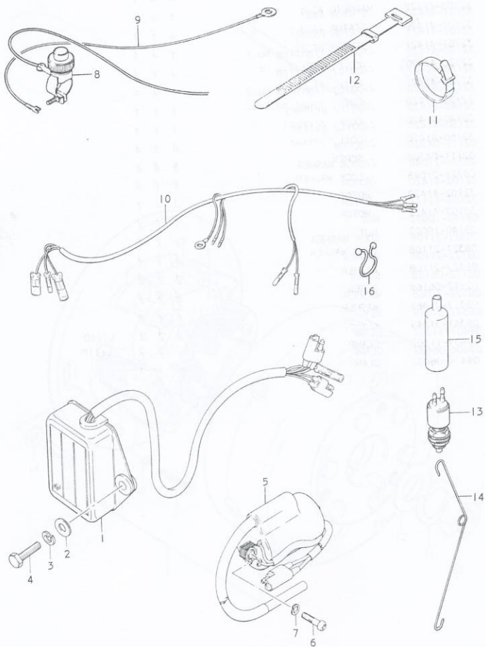
FIG.15 ELECTRICAL
