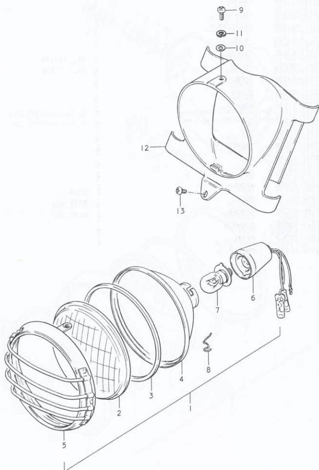
FIG.20 HEADLAMP (PE250C·PE250N)
