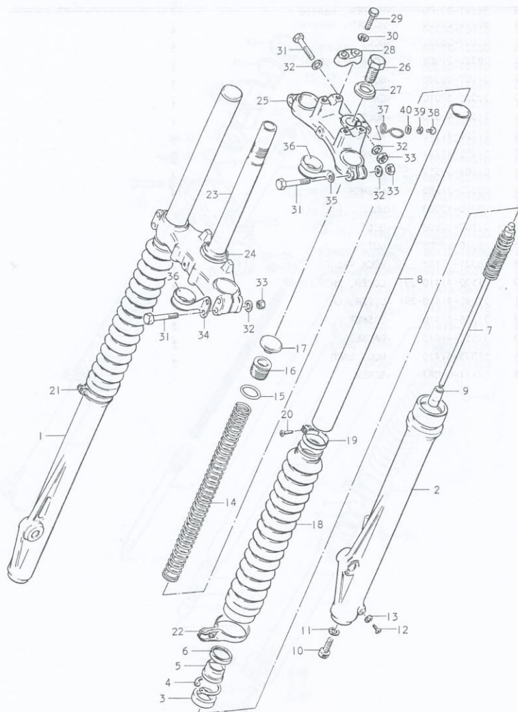
FIG.31 FRONT FORK (PE250C·PE250N)
