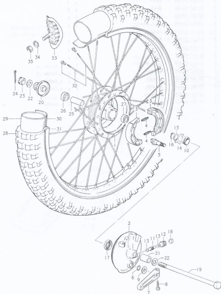
FIG.34 FRONT WHEEL (PE250B)
