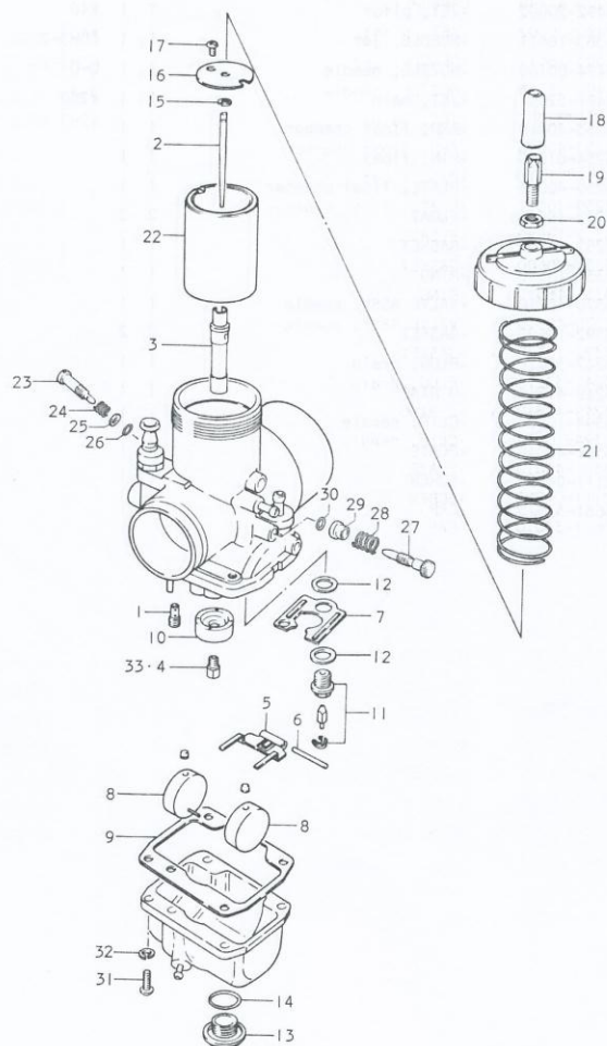
FIG.5 CARBURETOR (PE250B-PE250C)
