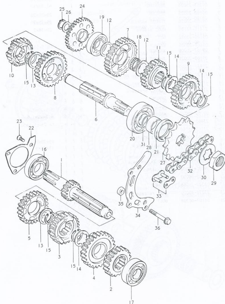
FIG.11 TRANSMISSION
