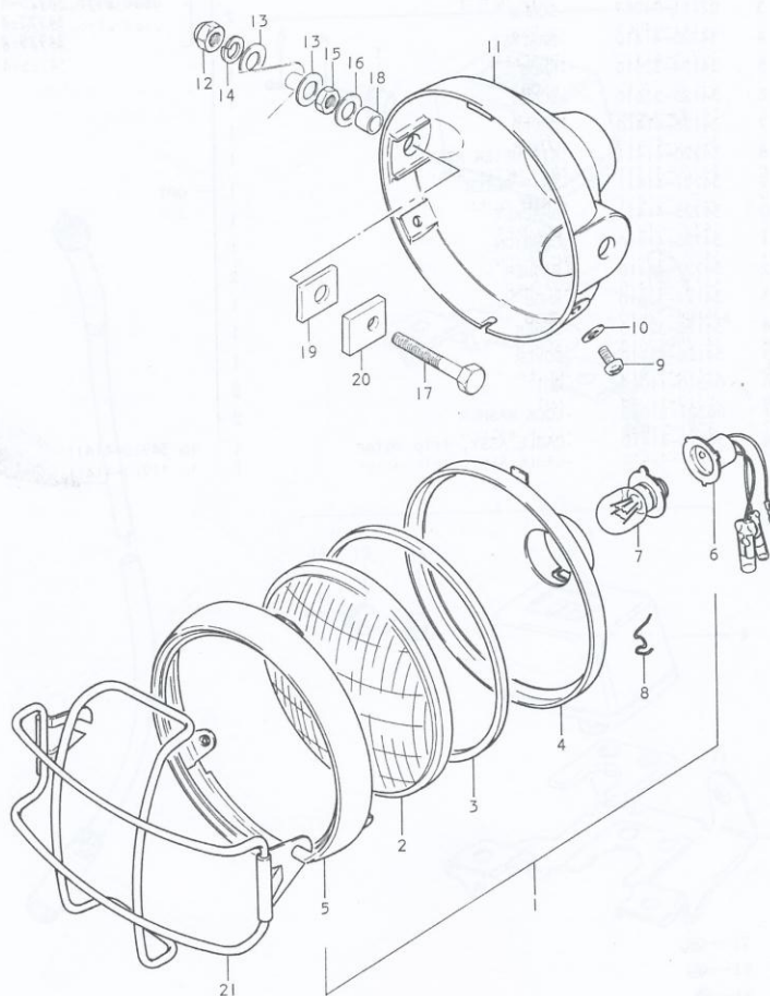
FIG.19 HEADLAMP (PE250B)
